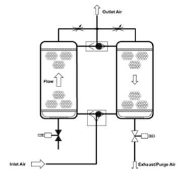
Figure 1 - PSA Process (Simplified)
