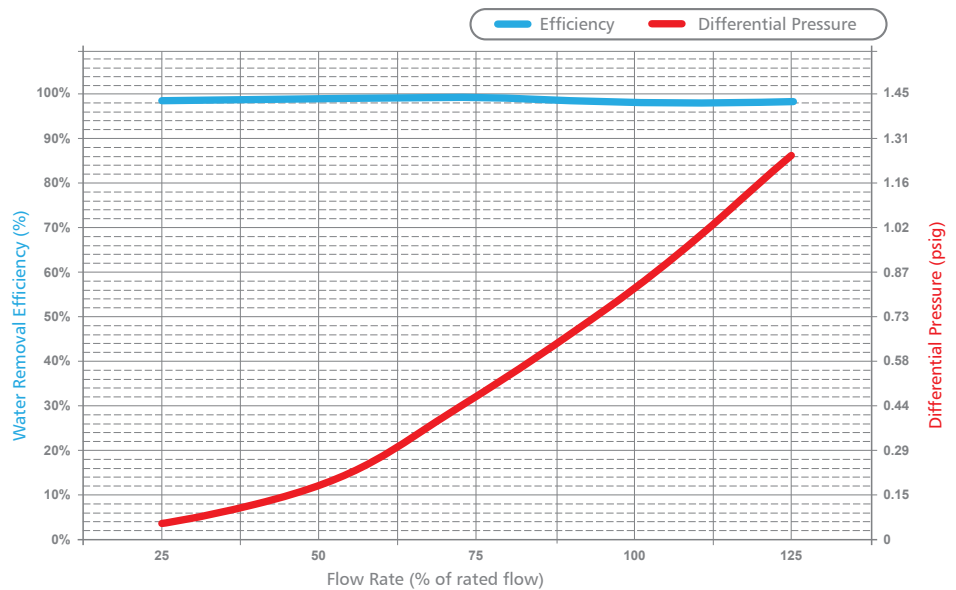
Actual results, using an NWS 070 tested to ISO 12500-4 standards.
